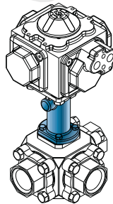
Fugitive Emission With Actuator
