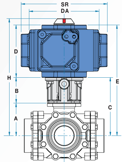
3" - 4" (DN80-DN100)
